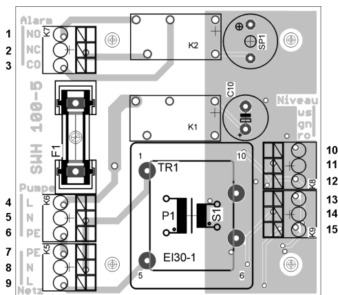
Plan de raccordement
