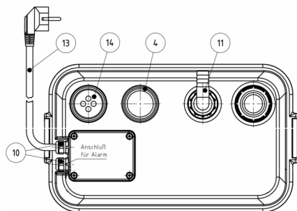
Plan de raccordement
