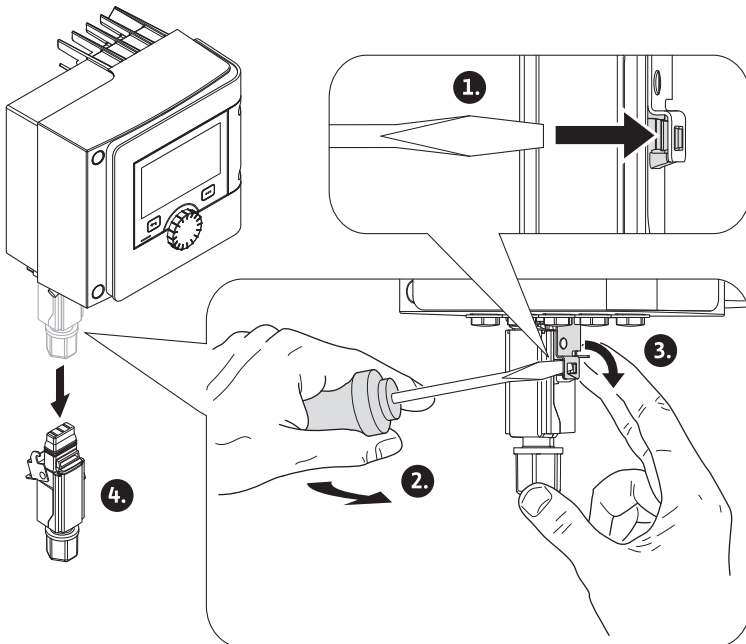
Fig. 12: Wilo-Connector demontieren
