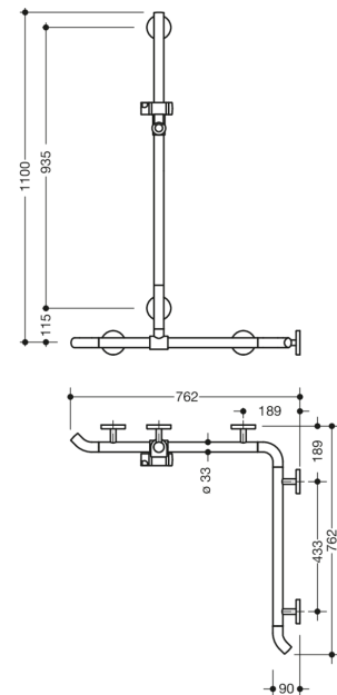
Abmessungen in mm
